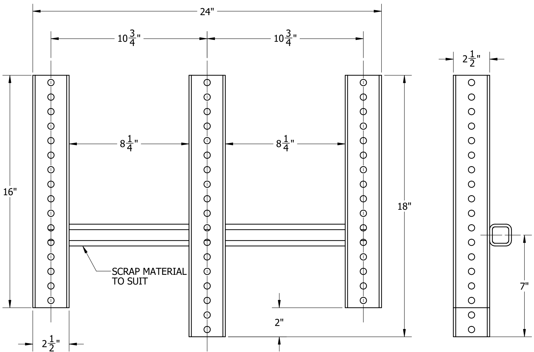
OUTER SLEEVE ASSEMBLY
